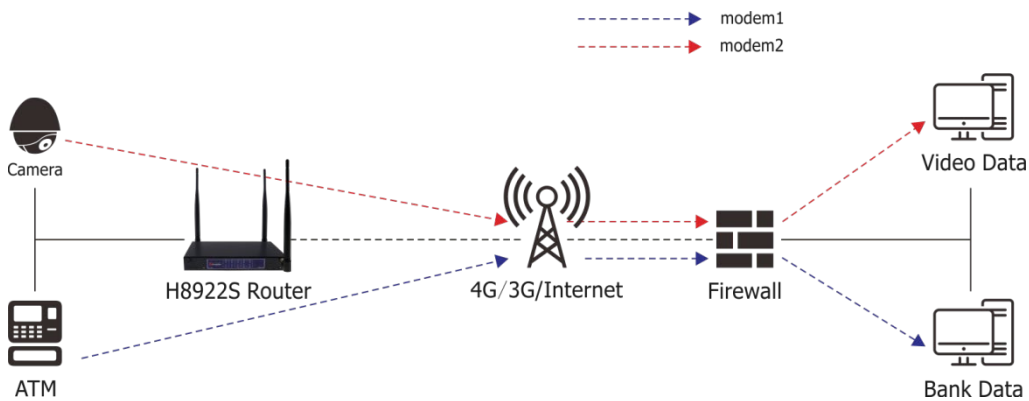
Figure 1-2 Schematic diagram of Dual Mode Online Application
