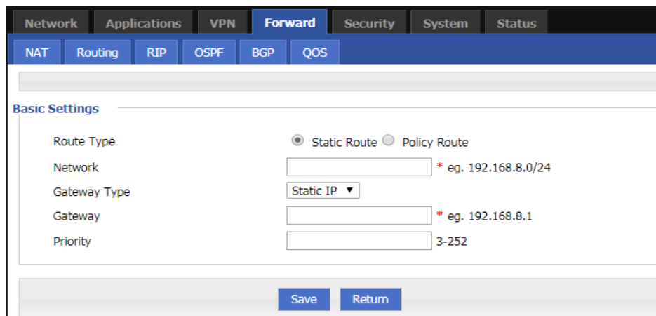
Figure 5-47 The configuration page of Static Routing
