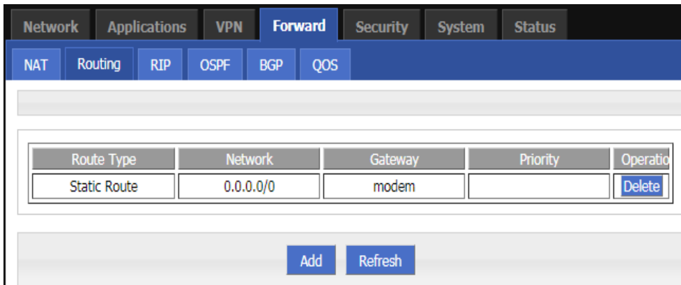
Figure 5-46 The configuration page of “Routing”
