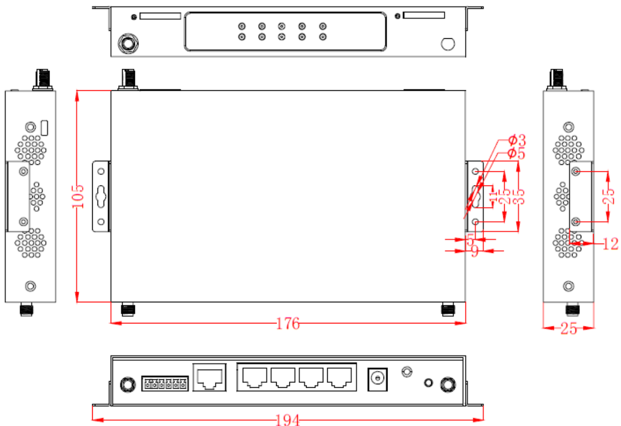
Figure 2-2 H8922S 4G router views
