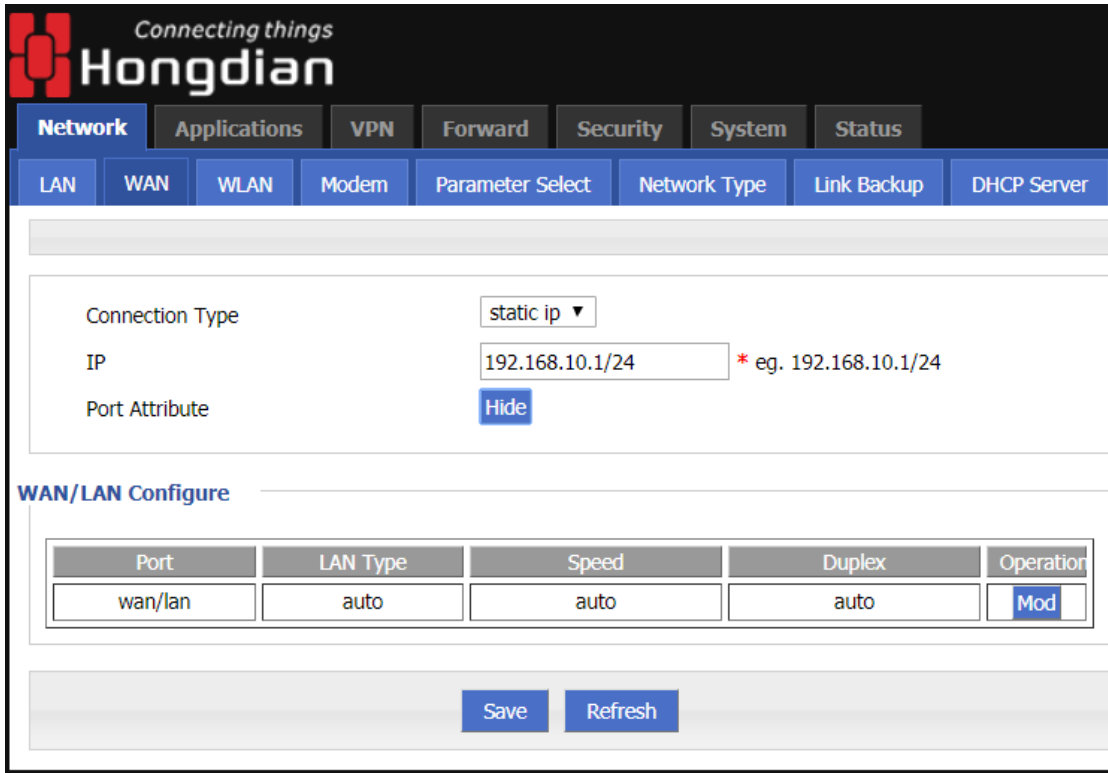
Figure 5-4 The page of WAN
