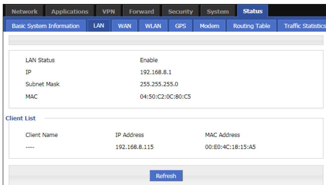
Figure 5-84 The page of "LAN"
