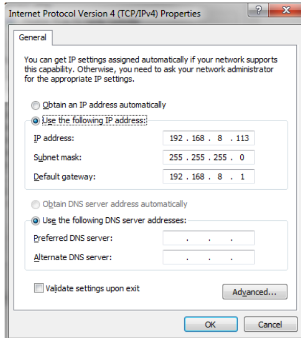
Figure 4-4 Internet Protocol (TCP/IP) Properties Window
