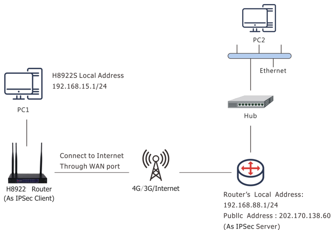
Figure 6-9 Establishing IPSec communication
