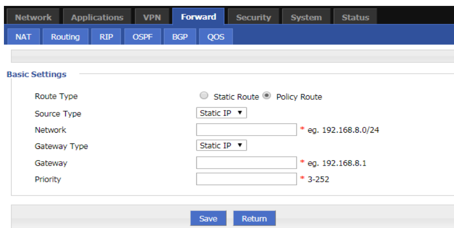
Figure 5-48 The configuration page of Policy Routing
