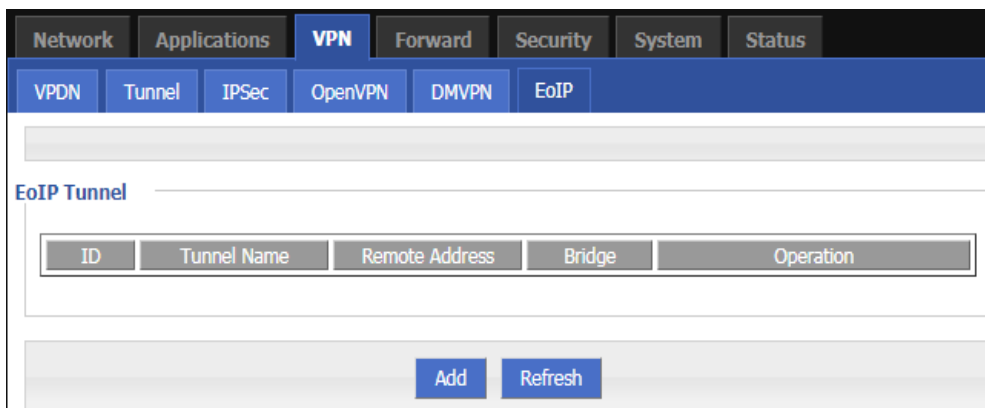
Figure 5-68 The page of "EOIP"
