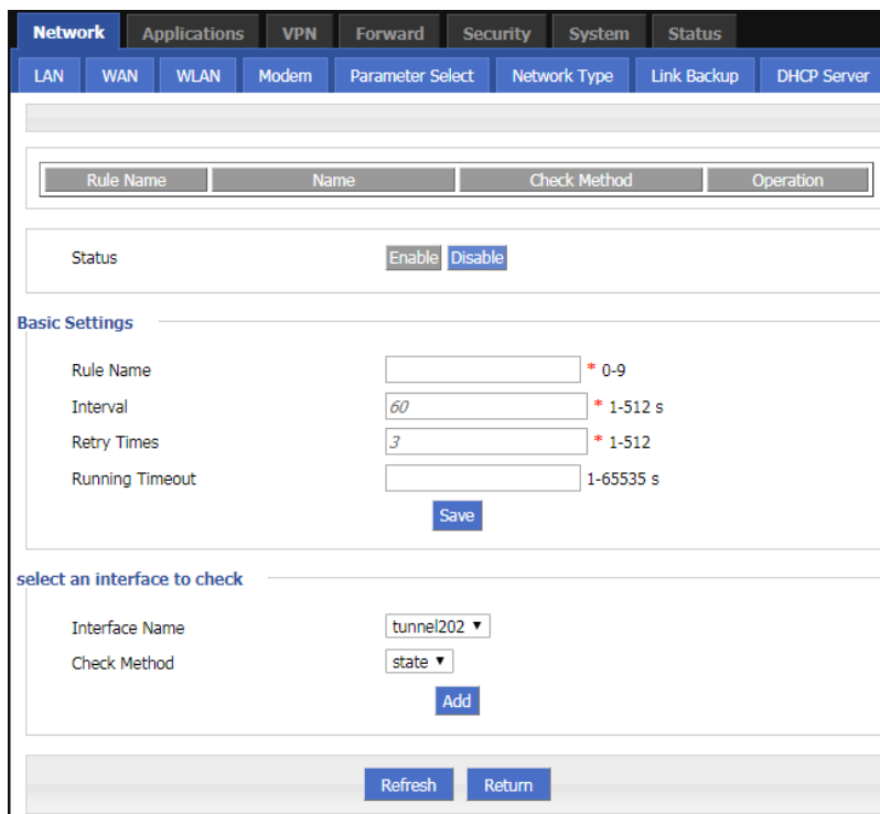
Figure 5-12 The configuration page of “Parameter Select”
