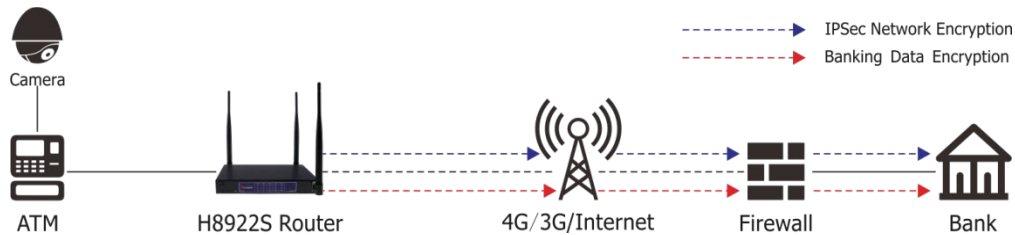
Figure 1-1 Network structure
