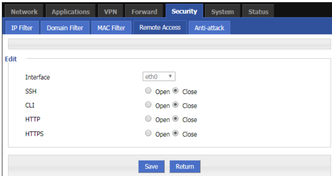
Figure 5-38 The editing page to open Ports
