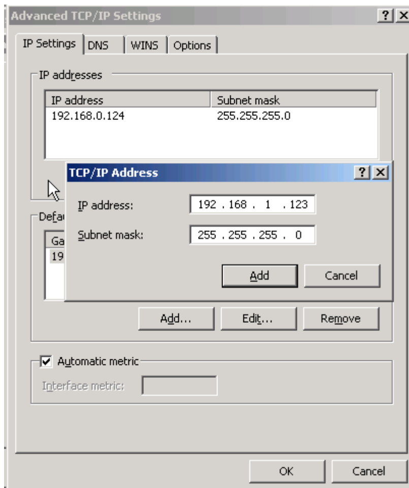
Figure 5-77 Add an IP address
